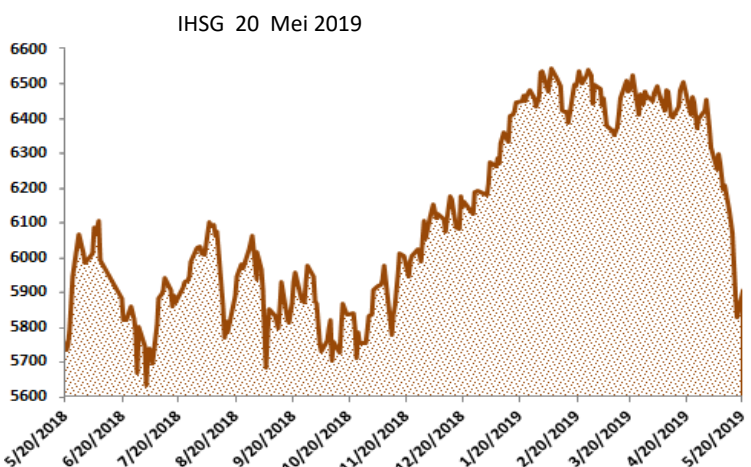
IHSG Statistics
