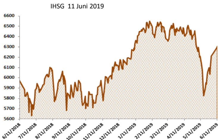
IHSG Statistics
