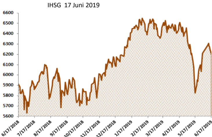
IHSG Statistics
