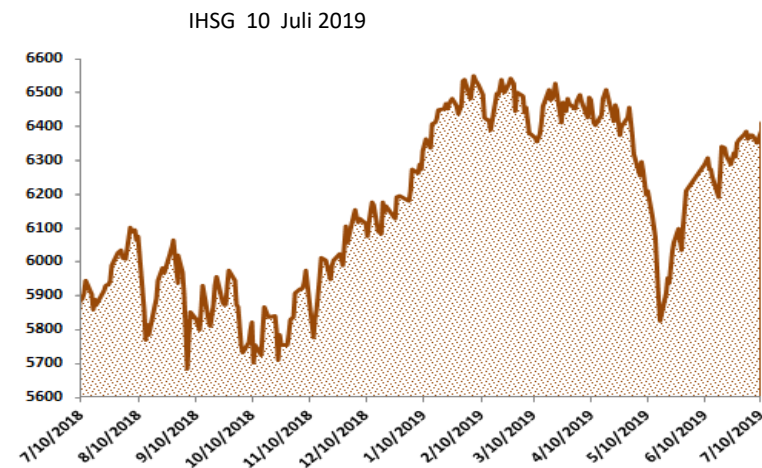
IHSG Statistics
