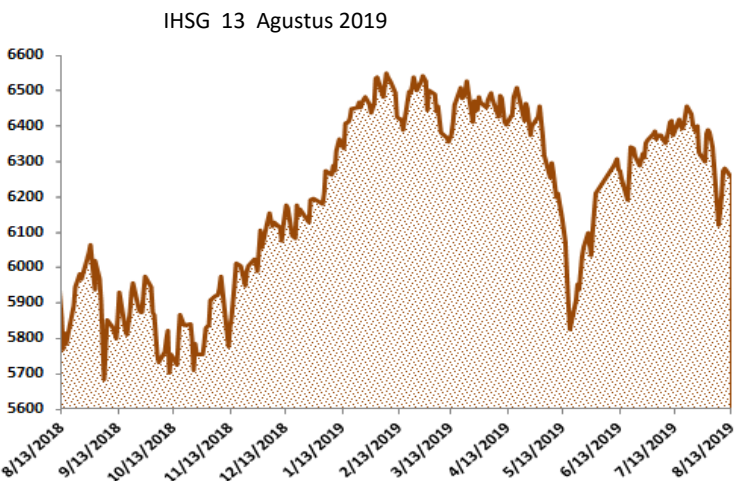
IHSG Statistics
